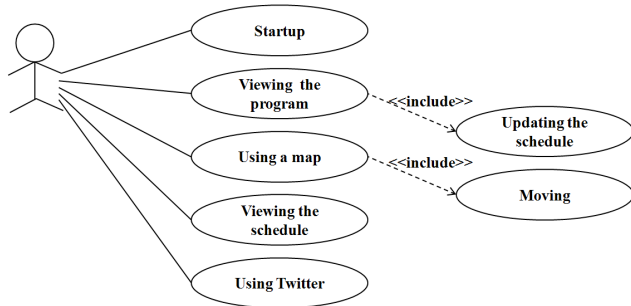
Figure 1. Use case diagram for the conference guide system
