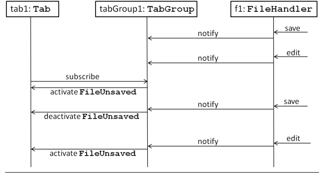
Figure 3. Dynamic subscription and layer activation
