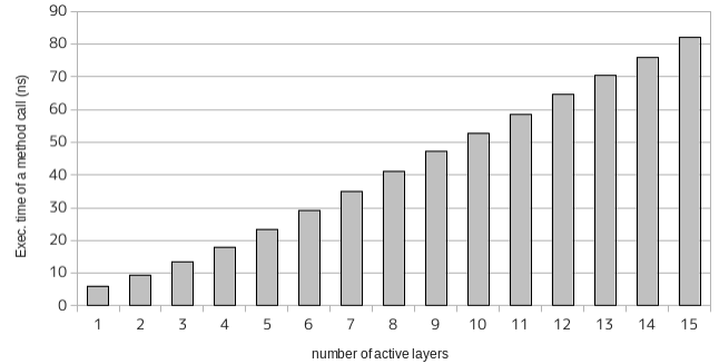
Figure 12. Execution time of a method call in ServalCJ when increasing the number of active layers. We ran the benchmarks 10 times; the range of error was approximately 0.04% – 0.1%.
