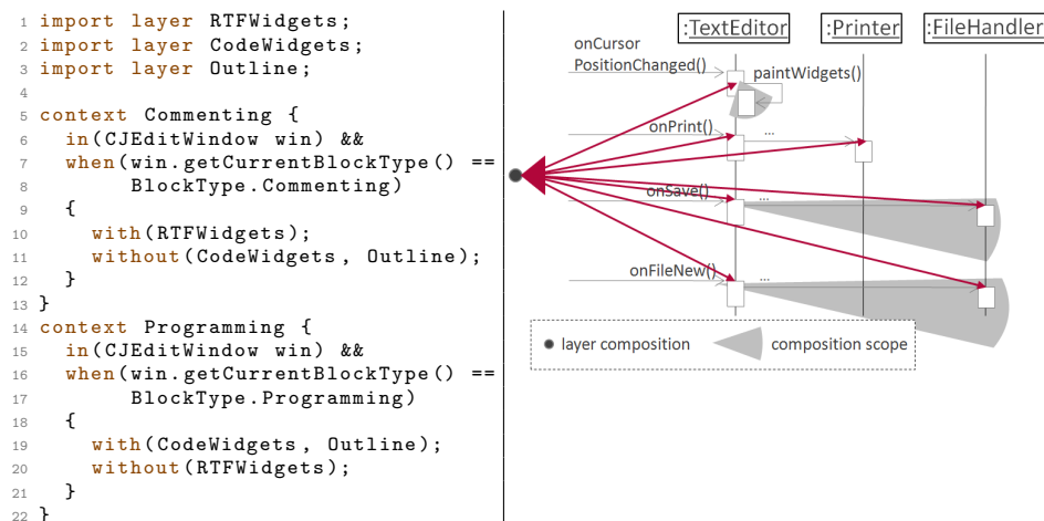
Fig. 6. Using the when predicate in CJEdit.
