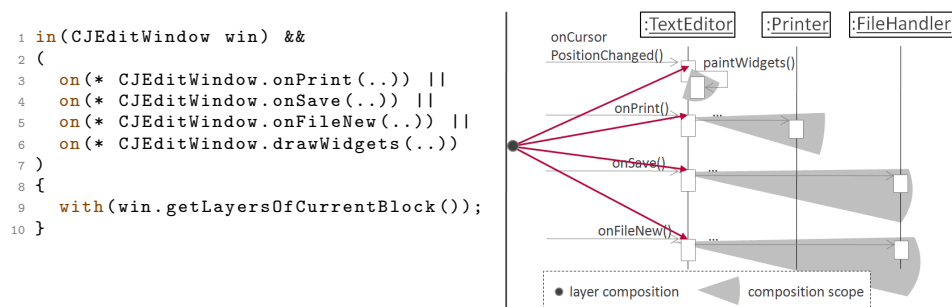
Fig. 5. Using the on predicate in CJEdit.
