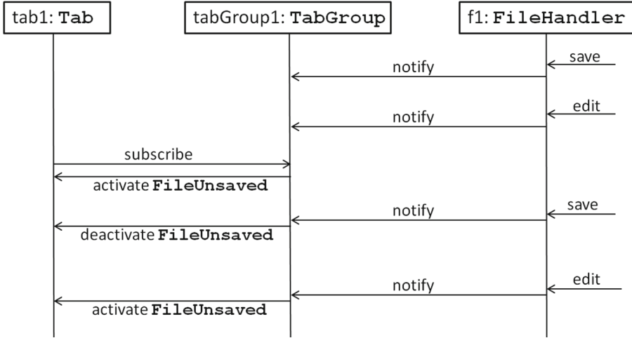
Fig. 3. Dynamic subscription and layer activation
