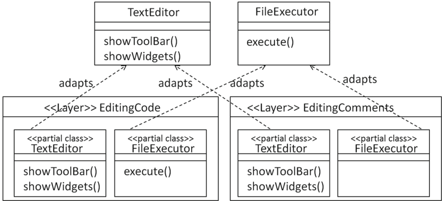
Fig. 1. Relationships among layers and classes
