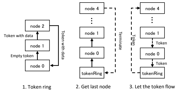
Figure 6. Behavior of token ring
