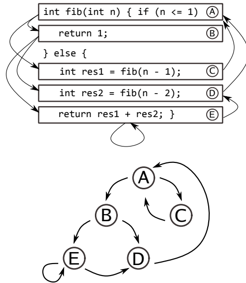
Fig. 2: The Fibonacci function and its control flow.
